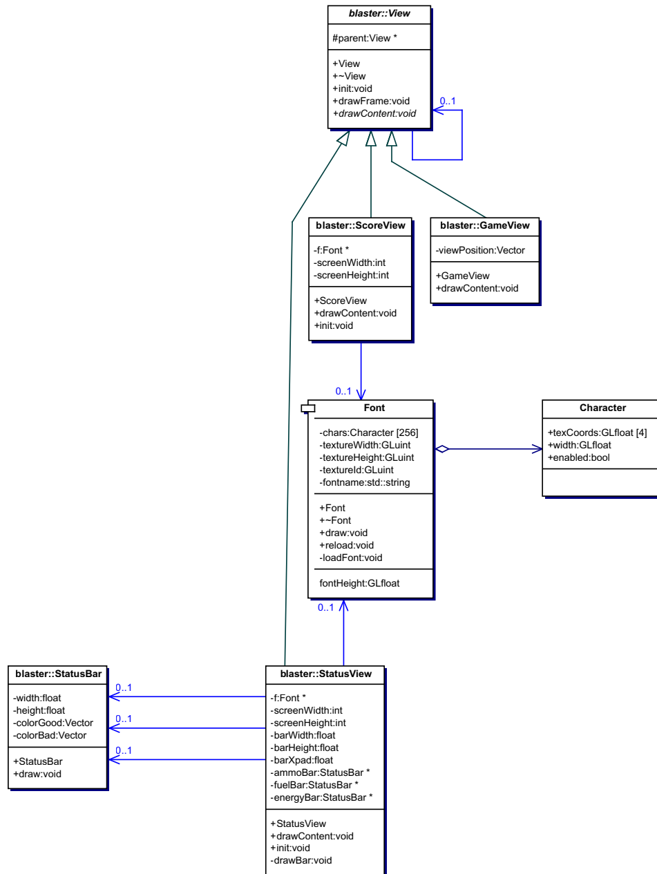
Figur A.7: UML diagram over views
