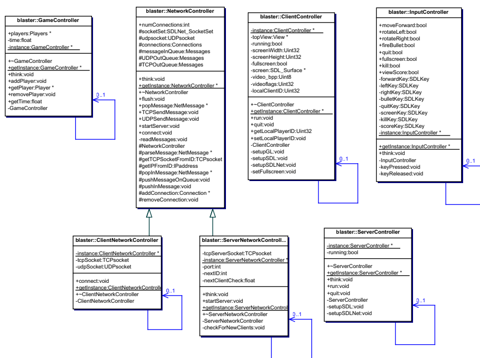
Figur A.2: UML diagram over controller delen
