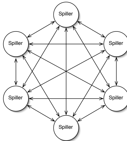
Figur 5.1: Peer to peer modellen
