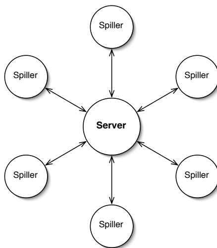
Figur 5.3: Klient-server modellen
