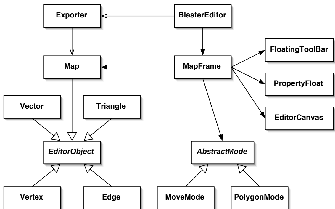
Figur A.8: Klasse diagram over editoren
