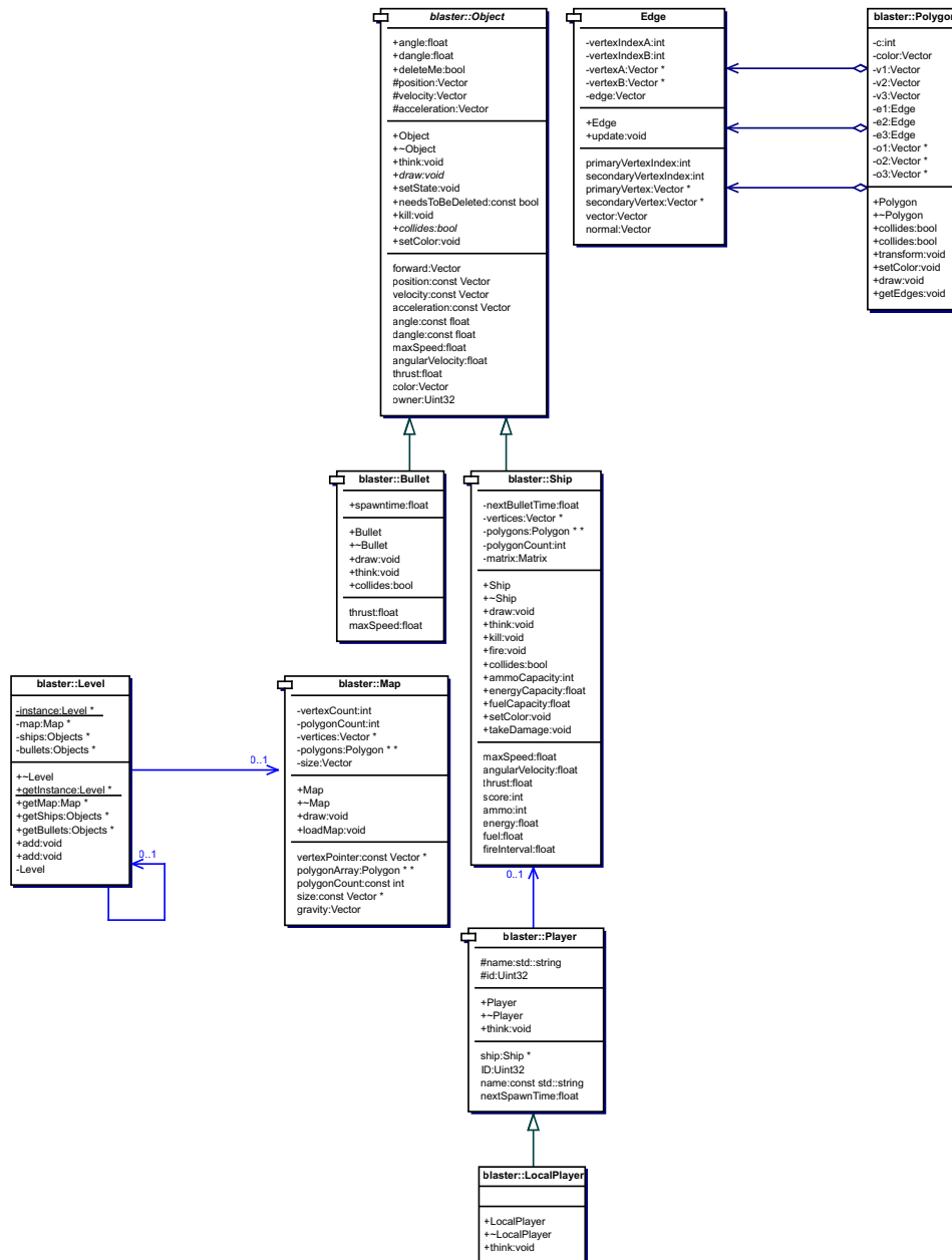
Figur A.3: UML diagram over model delen
